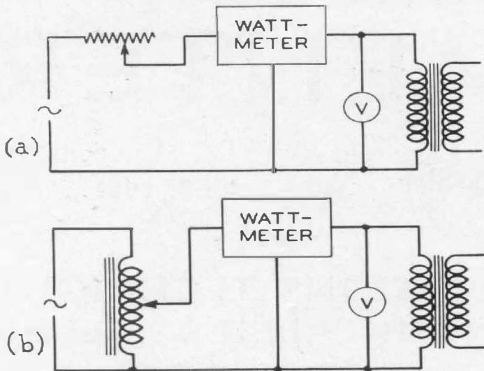
FIGURE 1. (a) Circuit for measuring the no-load loss of a power transformer using a series rheostat to vary line voltage. (b) Similar circuit using the VARIAC
