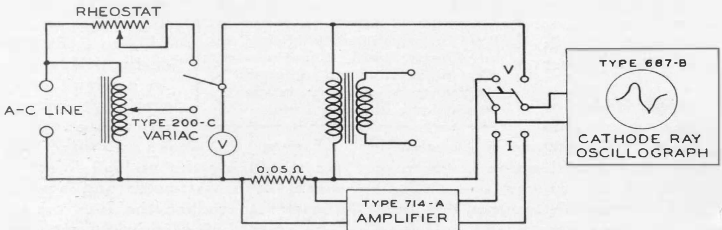
FIGURE 3. Circuit used to obtain the oscillograms of Figure 4 and Figure 5. The 0.05-ohm resistor supplies a voltage drop which is amplified to obtain the current wave shape
