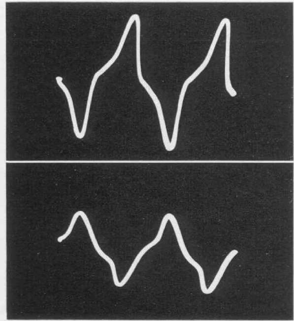
FIGURE 5. Voltage (upper) and current (lower) when the rheostat is used. Both curves are non-sinusoidal and the current is lower than in Figure 4
