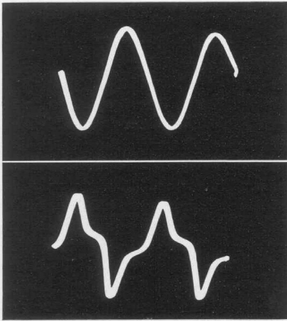
FIGURE 4. Voltage (upper) and current (lower) in the transformer primary when the VARIAC is used. The voltage is sinusoidal and the current distorted
