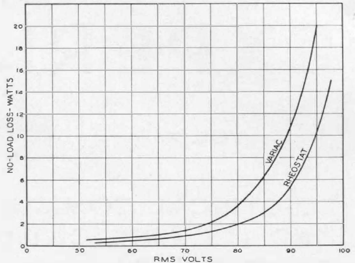
FIGURE 2. Power loss curves obtained by measurement using the circuits of Figure 1. Note that the results differ by 50%
